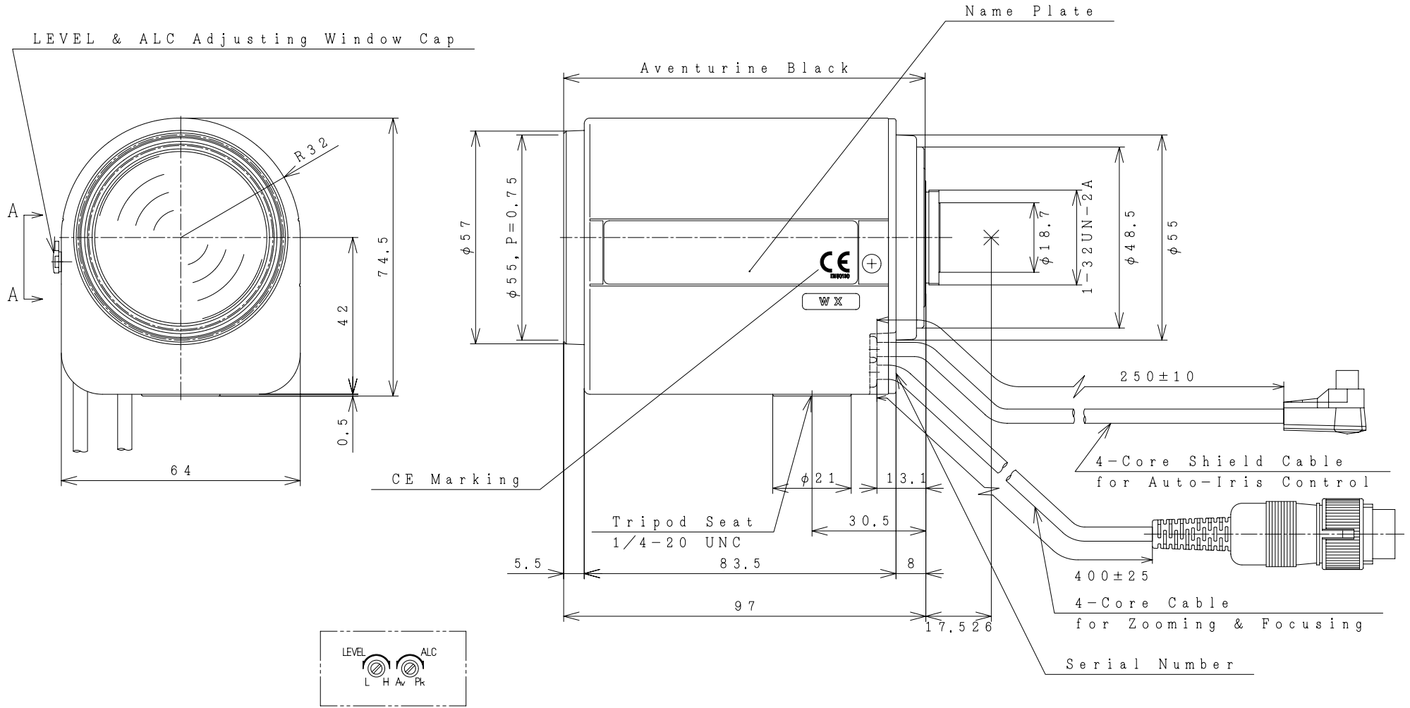
A-A (When Cap is off)
