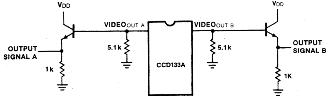
Fig. 2 TEST LOAD CONFIGURATION
