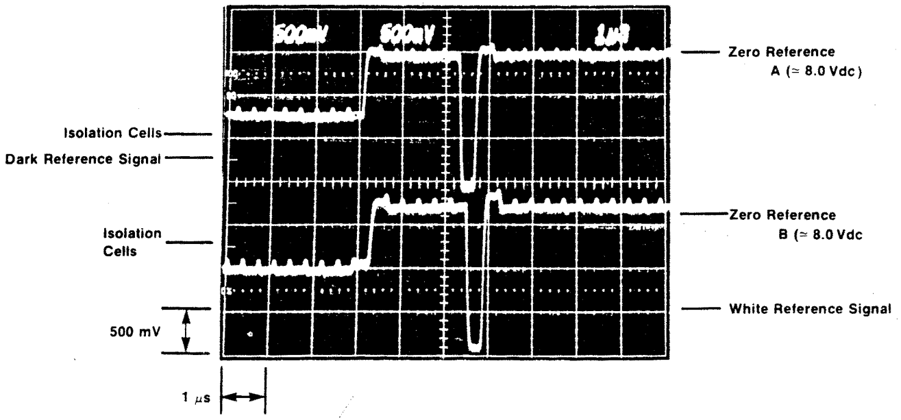
End of One Scan Video Output
